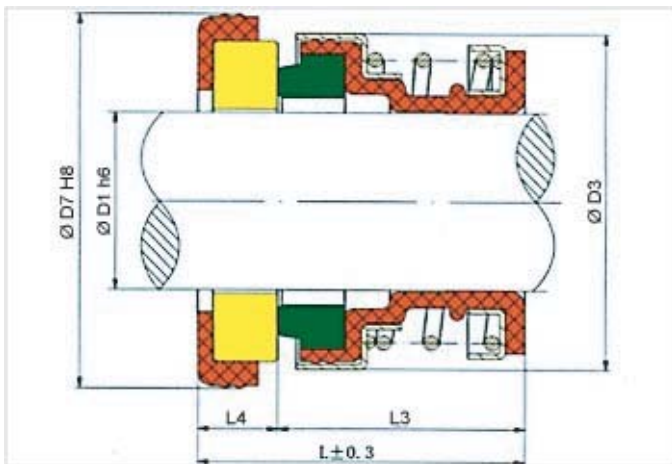
Mechanical seal structure ZY-103
