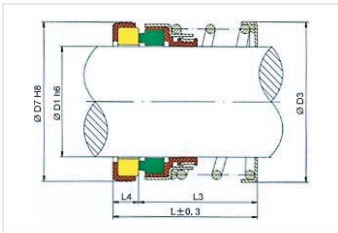
Mechanical seal structure ZY-108
