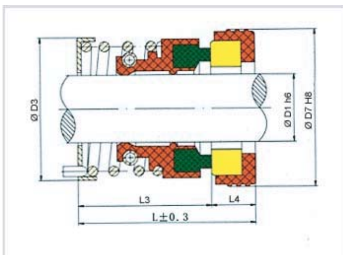
Mechanical seal structure ZY-156
