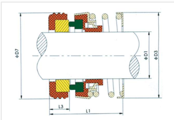
Mechanical seal structure ZY-166T
