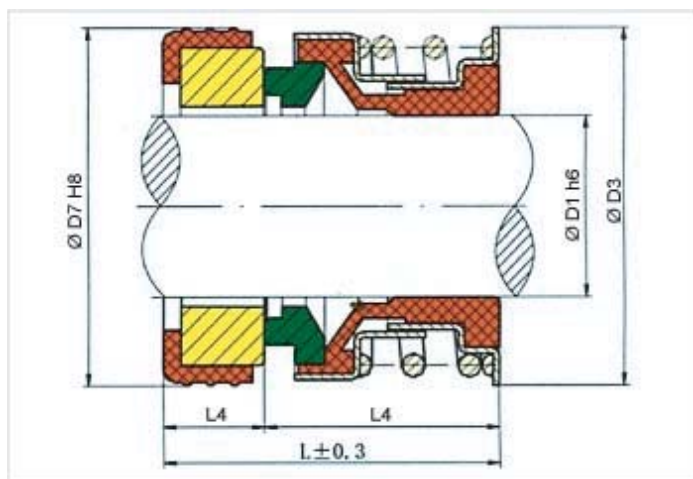
Mechanical seal structure ZY-166
