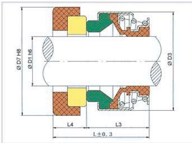
Mechanical seal structure ZY-301
