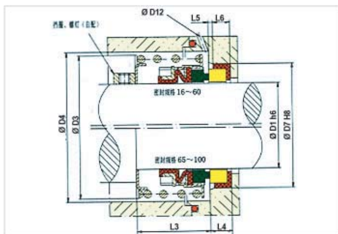
Mechanical seal structure ZY-580
