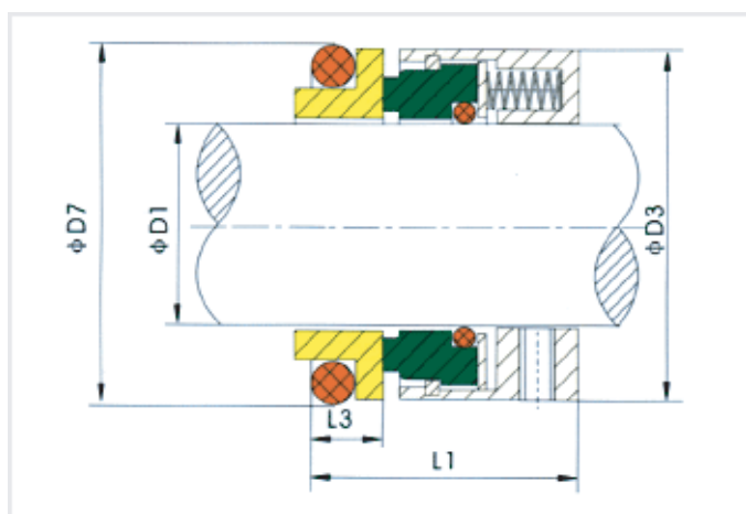
Mechanical seal structure ZY-58U
