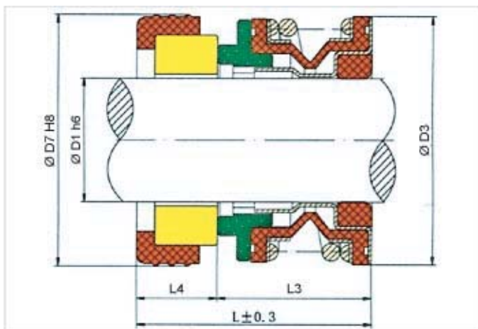
Mechanical seal structure ZY-E
