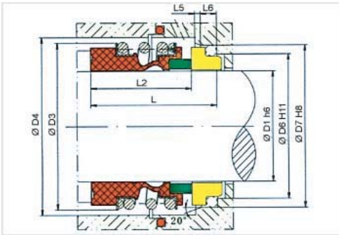
Mechanical seal structure ZY-G2
